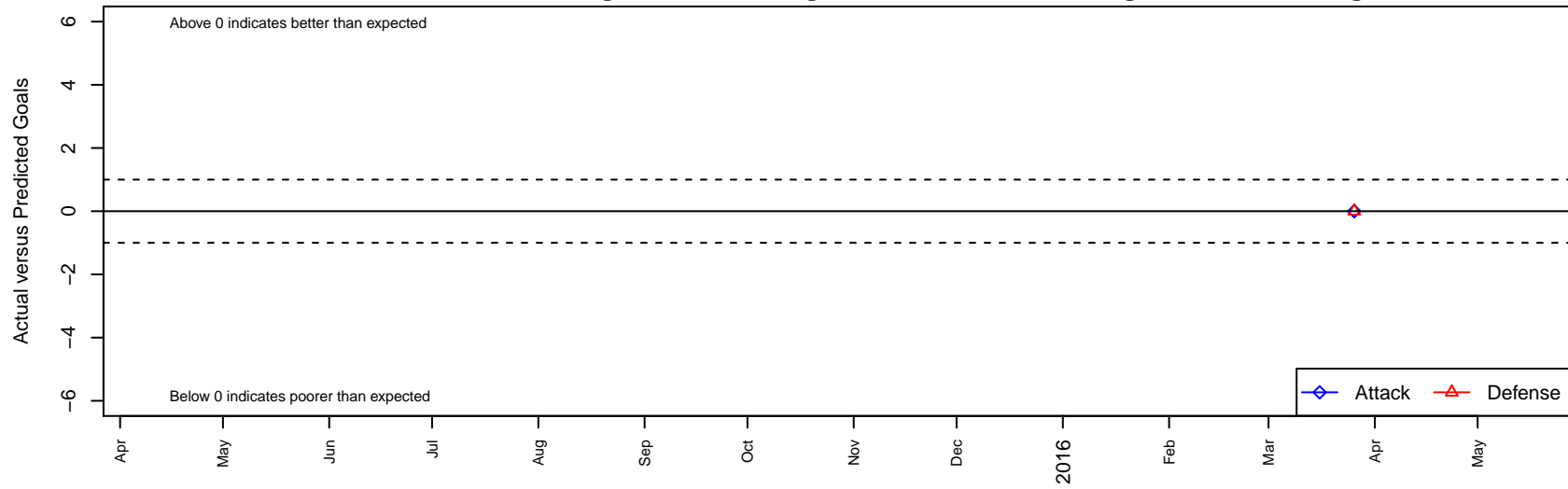
Surrey United 1998G Dots are actual minus expected GF (blue circles) and GA (red triangles). Blue line is smoothed change in attack strength. Red is smoothed change in defense strength.
